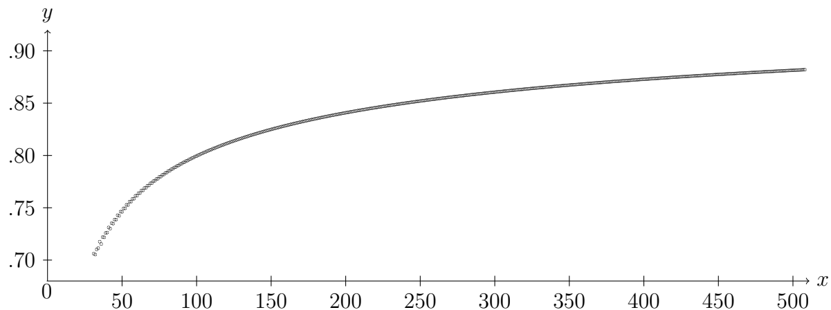
Figure 1: Plot of the values of \frac{\ln f(n)}{(6n)^{1/3} \ln[(6n)^{1/3}]} for 31 \leq n \leq 508 .
